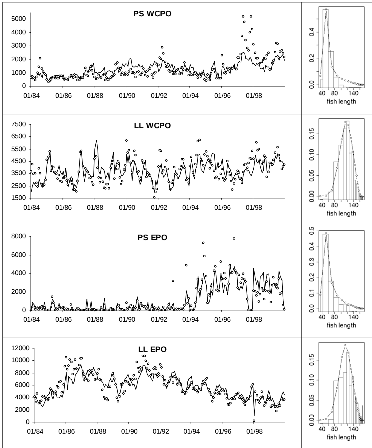
Figure 3: Comparison of observed (circles) and predicted (lines) catch series and size frequency distributions aggregated by main categories of fleets (PS = purse seine, LL = longline) in the western central (WCPO) and eastern Pacific Ocean (EPO).
