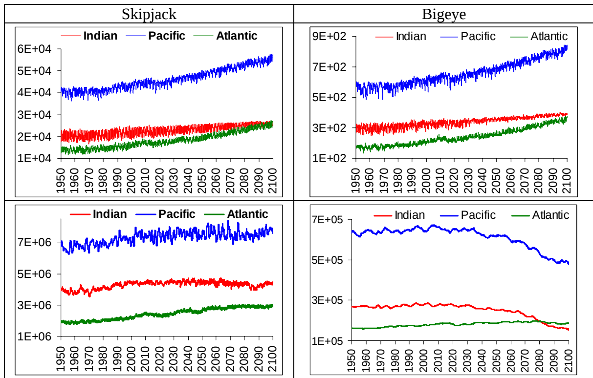
Figure 6. Trends by ocean of bigeye and skipjack larvae (top) and adult (bottom) biomass (million tonnes) estimated by SEAPODYM under the IPCC SRESA2 scenario.
