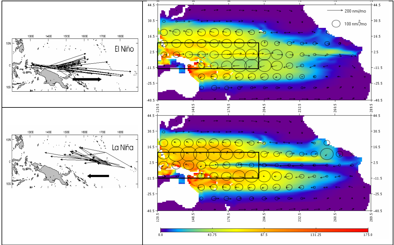
Figure 4: Distribution of biomass of a skipjack cohort at the first month after the age of maturity in November 1997 (El Niño phase) and November 1998 (La Niña phase) in the Pacific Ocean. Circles and arrows represent random (diffusion) and directed (advection) movements of population density, respectively, and are averaged by 10 degree squares. Black rectangles show the region where tags have been released and recaptured during the earlier corresponding ENSO phases (redrawn from Lehodey et al., 1997).
