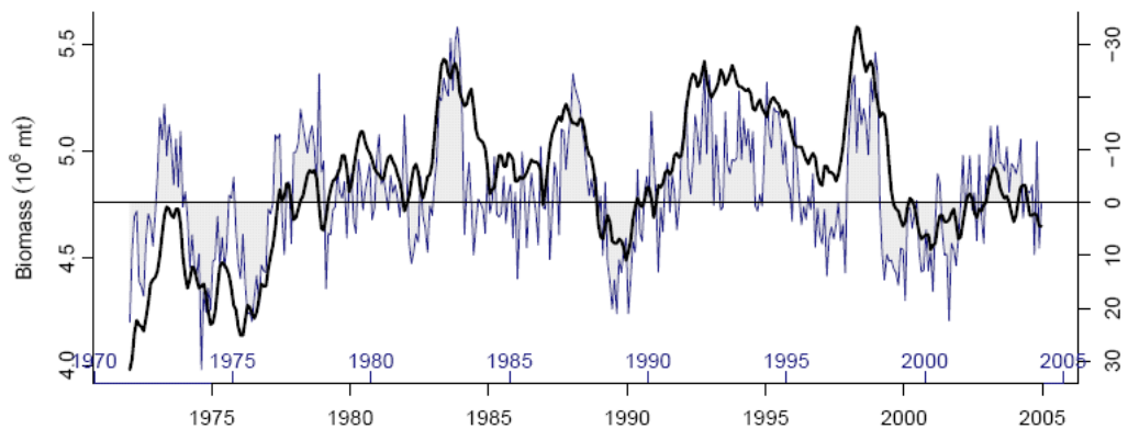
Figure 5: Biomass of young skipjack tuna (sum of ages from 3 month to 3 quarter) and eight month lagged Southern Oscillation Index (notice that y axis is inverted) as an indicator of El-Nino event (Redrawn from Senina et al., in press ).
