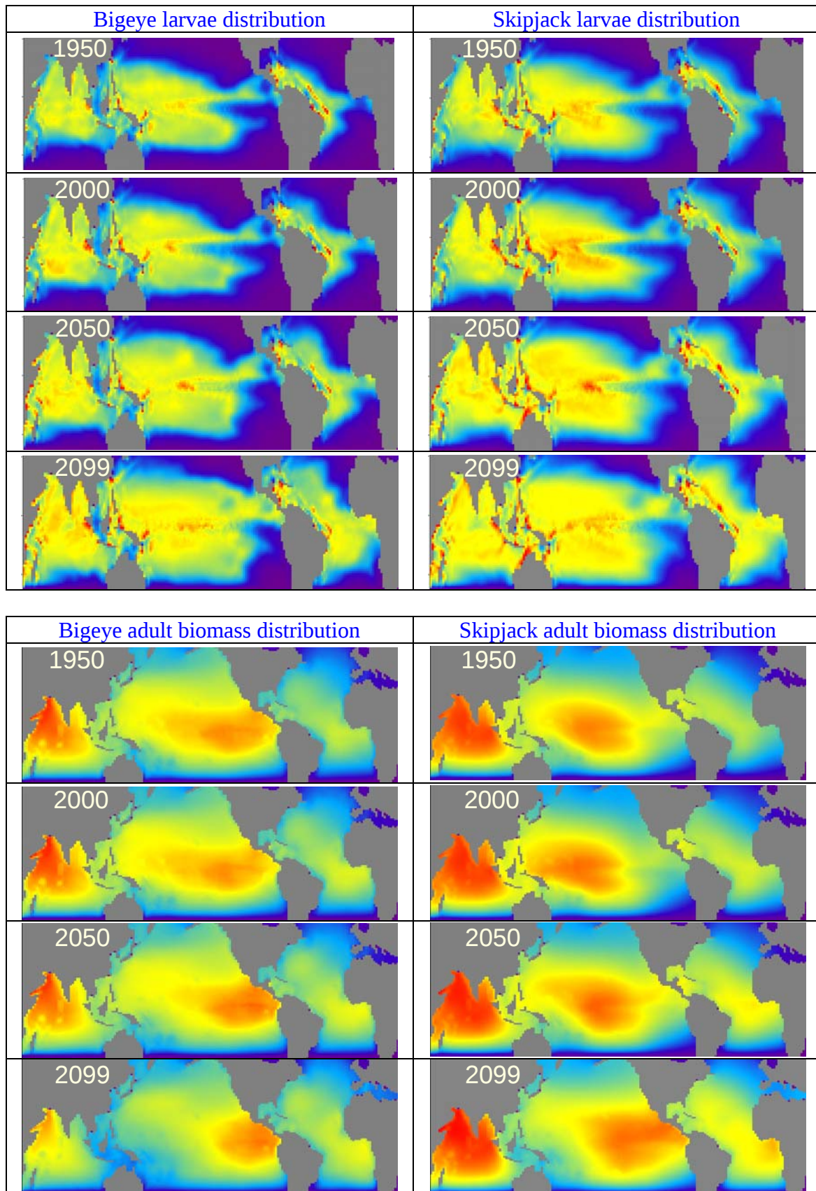
Figure 7. Change in spatial distribution of bigeye and skipjack larvae and adult biomass under the IPCC (SRES A2) scenario. Note that parameter optimization is carried out in the Pacific Ocean for the period 1985-2004). Fishing impact is not included in this simulation.
