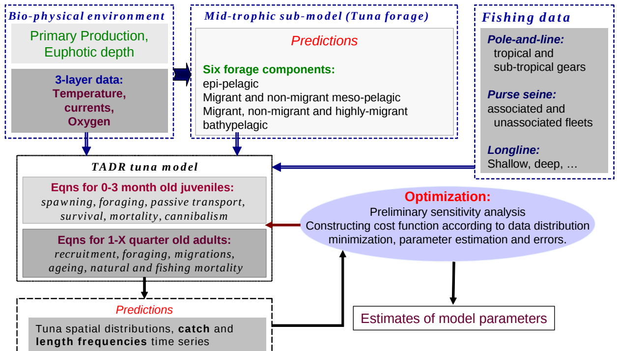
Figure 1: General scheme of the SEAPODYM model with optimization approach.
