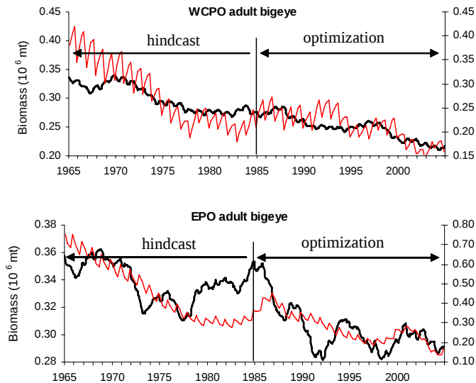
Figure 2: Trends in Pacific bigeye tuna population predicted in WCPO and EPO with optimization (1985-2004) and hindcast prediction to 1965 for experiment based on ESSIC (black thick line) forcing fields. The trends for adults are compared to estimates (thin red line) from stock-assessment model MULTIFAN-CL (Hampton et al. 2006, Sibert et al. 2006).
