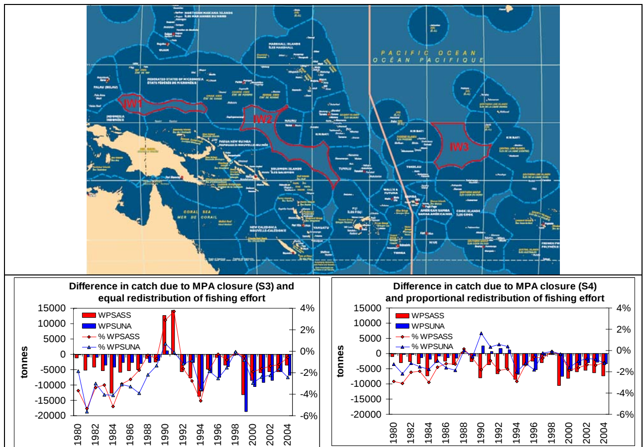
Figure 8: Location of the three MPAs considered in the simulation and results showing the difference in skipjack catch by purse seine fleets due to the MPA closures and two different scenarios dealing with released fishing effort – either to redistribute the effort equally among other enclaves (S3) or proportionally to the existing distribution (S4).
